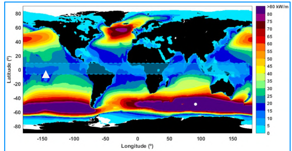
30-year average wave power (1989-2018) – ERA5 database
